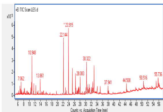
Figure 2: Gas Chromatogram of Lannea egregia twig essential oil
