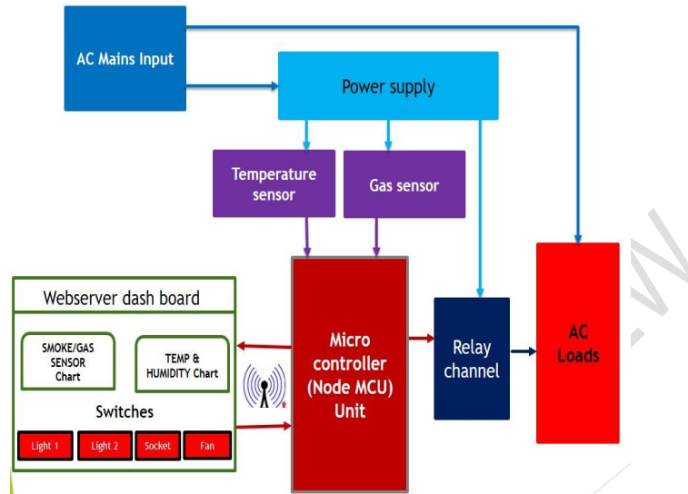
Fig.1 Block diagram of the smart home automation system
