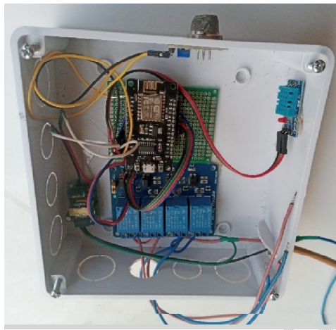
Fig. 5. Complete prototype of the Smart Home automation system
