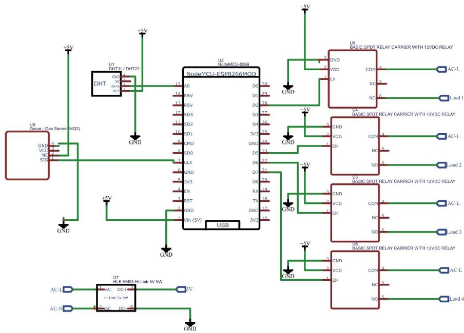
Fig. 3 Schematic diagram of the whole system
