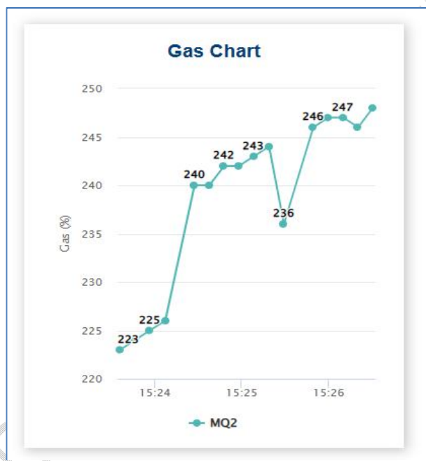
Fig. 7. Real-time measurement of smoke concentration in the air from the dashboard display
