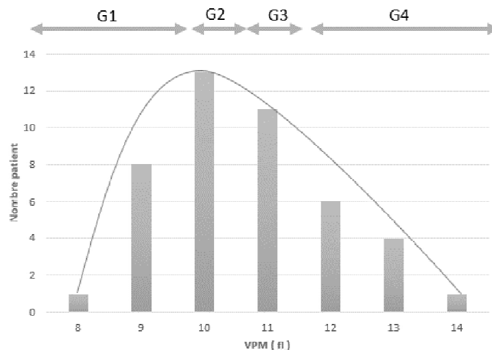
Figure 1: Average VPM according to the 4 groups
