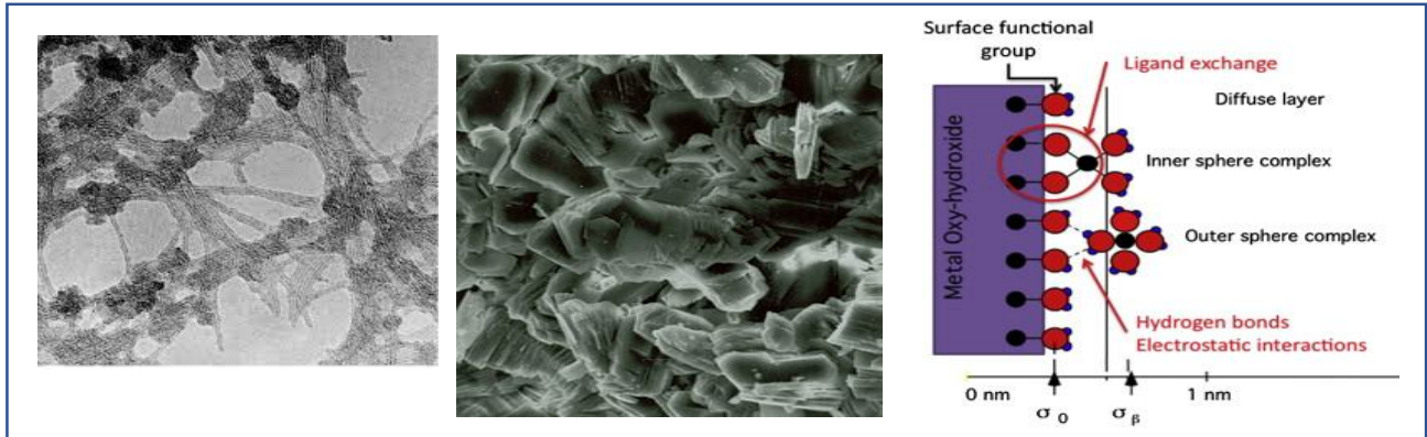
Fig 2- Clay minerals and dominant bonding mechanisms [13]
