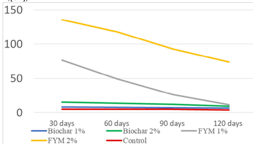
Fig 4- Carbon dioxide emission by different manures [64]
