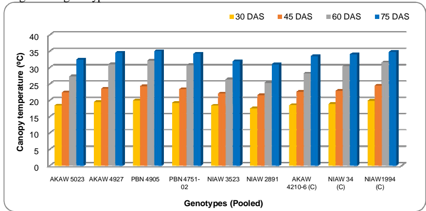
Fig 1. Canopy temperature
