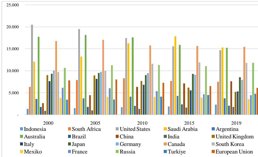
Figure 1. Carbon Dioxide (CO 2 ) Emissions from G20 Countries
