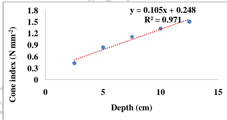
Fig. 3. Relation between cone index and depth
