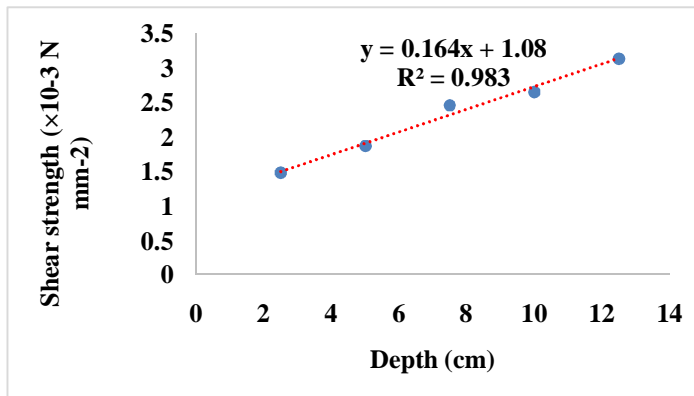
Fig.5.Relation between shear strength and depth
