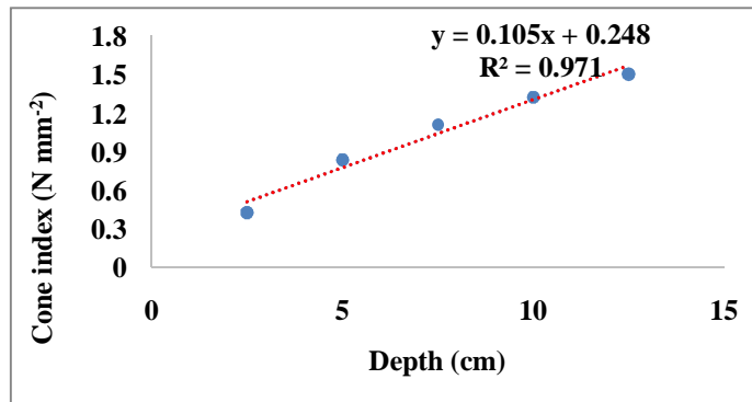
Fig.4. Relation between cone index and depth
