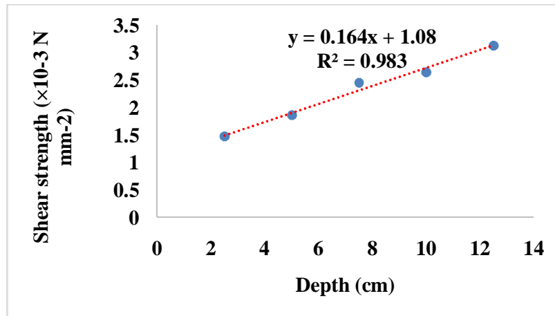
Fig. 5. Relation between shear strength and depth
