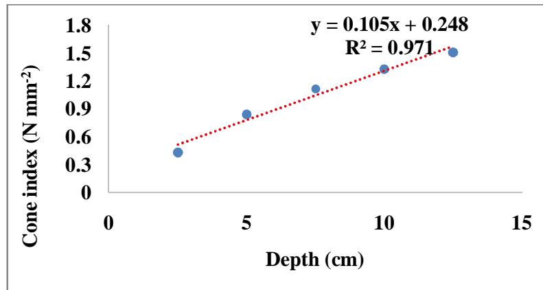
Fig. 4. Relation between cone index and depth
