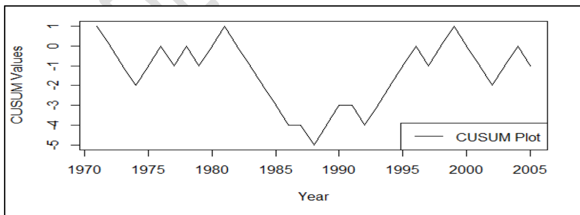
Figure 6: Distribution-free CUSUM plot for 24-hourly AMS rainfall intensity for Port Harcourt metropolis.
