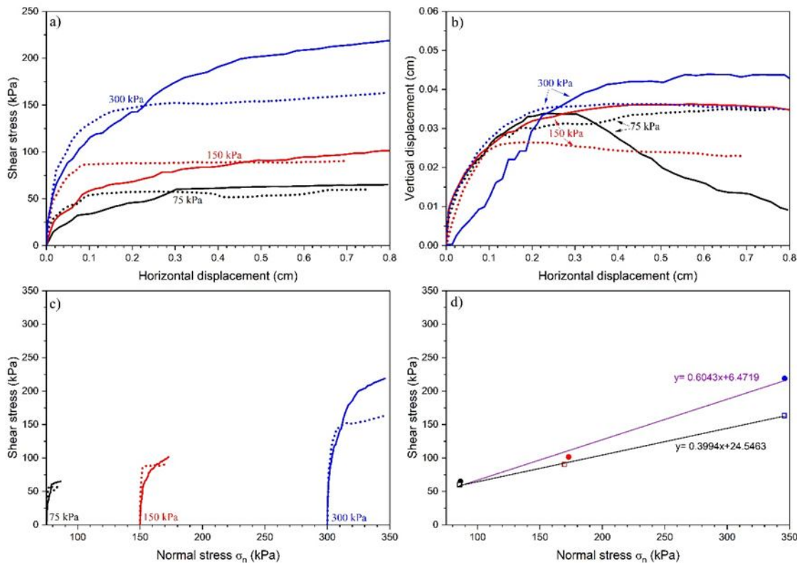
97 98 Figure 1: (a) Shear Stress (kPa) x Horizontal Displacement (cm), (b) Vertical Displacement (cm) x Horizontal 99 Displacement (cm), (c) Shear Stress (kPa) x Normal Stress (kPa) and (d) Mohr's wrap in the point 1 (dotted line) and 2 100 (solid line). The applied stresses of 75, 150 and 300 kPa are represented by black, red and blue, respectively.
