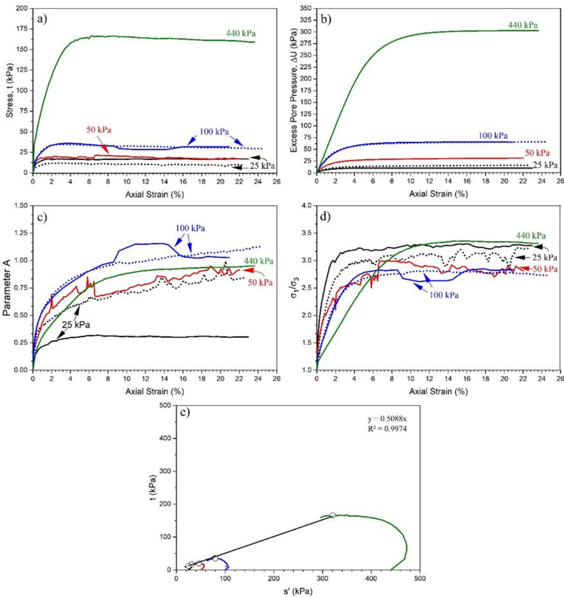
Figure 4: CIU Point 2 (a) Stress, t (kPa) x Axial Strain (%), (b) Excess Pore Pressure (kPa) x Axial strain (%), (c) Parameter A x Axial Strain (%), (d) Analyse \sigma_1/\sigma_3 (kPa) x Axial Strain (%) and (e) Mohr's wrap in the point 2. The applied stresses of 25, 50, 100 and 440 kPa are represented by black, red, blue and green, respectively. The solid line represents non-percolated samples and the dotted line percolated samples.
