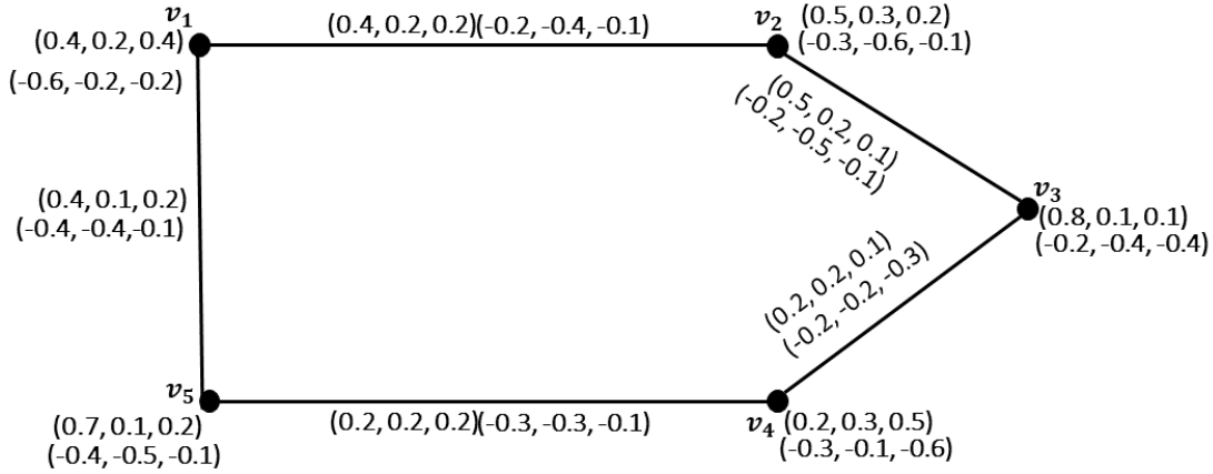
FIGURE 1. Bipolar Hesitancy Fuzzy Graph
