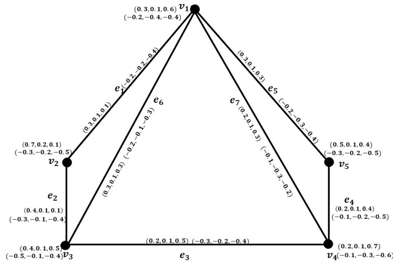
FIGURE 2. Secure Domination in BHFG
