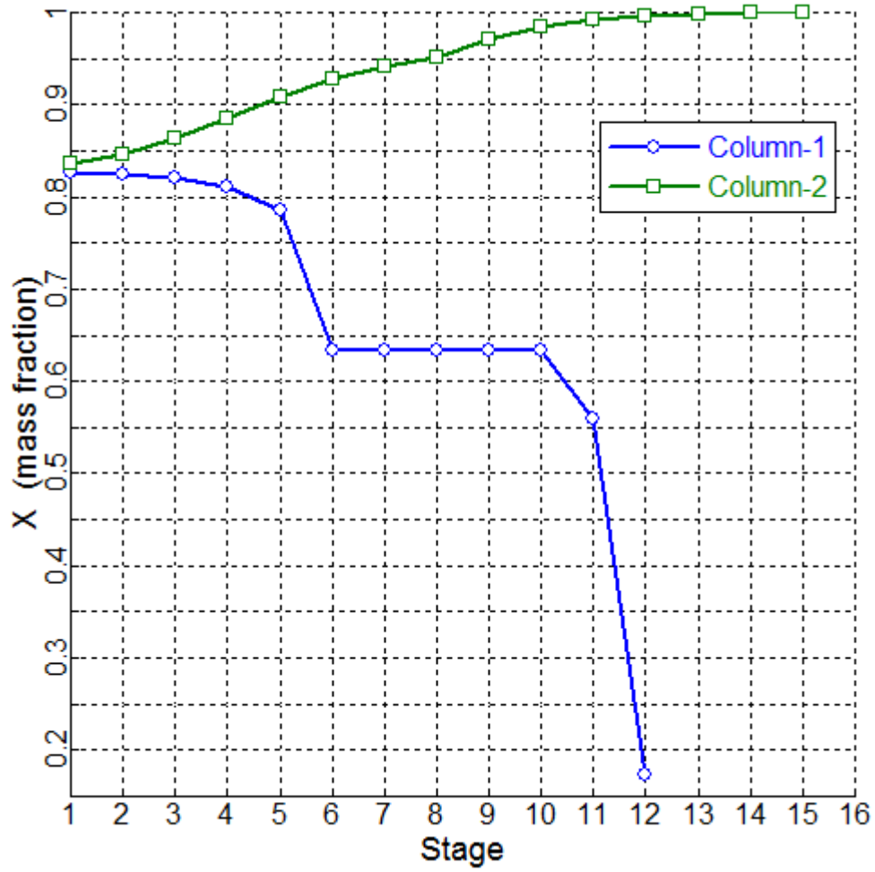
Figure 6. Liquid Composition Profile for Acetonitrile
