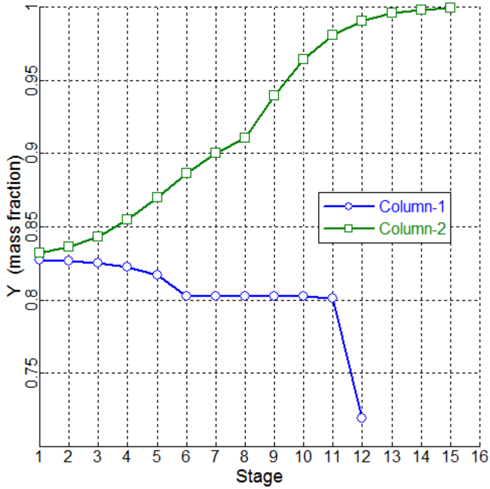
Figure 5. Vapor Composition Profile
