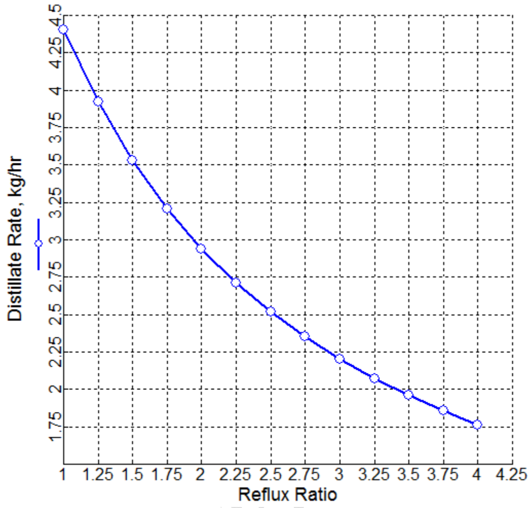
Figure 9. Variation of Distillate Rate with Reflux Ratio in Column-1
