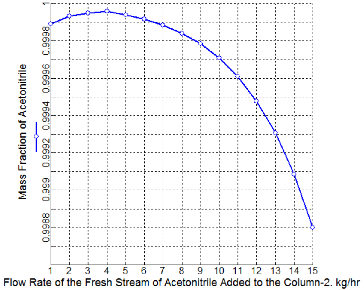
Figure 13. Variation of Mass Fraction of Acetonitrile with Flow Rate of the Fresh Stream of Acetonitrile Added to the Column-2.
