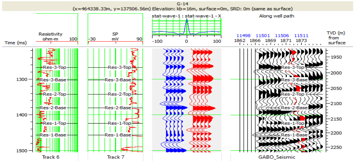
Fig. 15. Seismic well correction for G-14 showing extracted wavelet.
