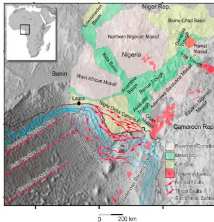
Fig. 2. Niger Delta map showing the main sedimentary basins and tectonic features [22].
