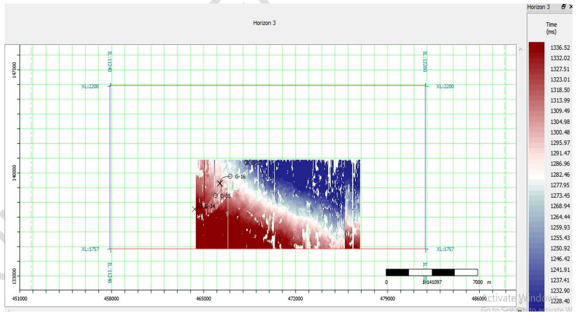
Fig. 14. Mapped result of the second Horizon (Horizon 3) on Inlines and Crosslines.
