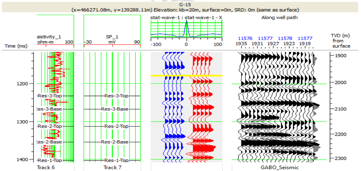
Fig. 16. Seismic well correction for G-15 showing extracted wavelet.
