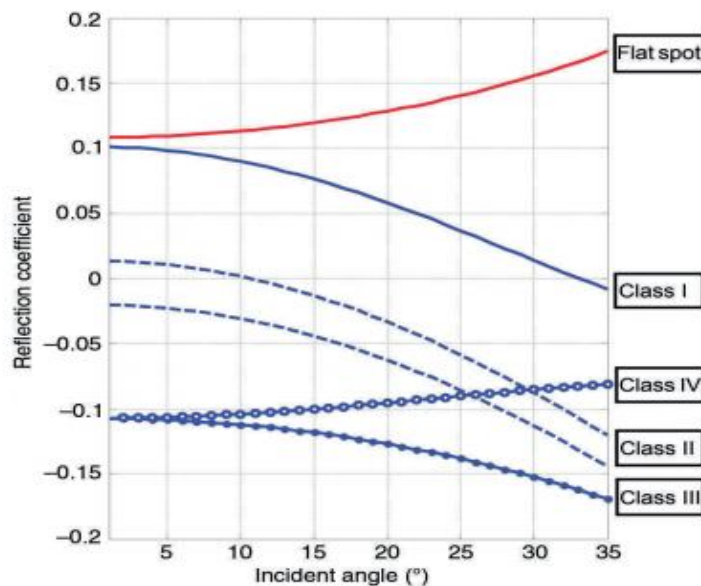
Fig. 3. The four AVO classes and the flat spot curve defined by [10, 30]
