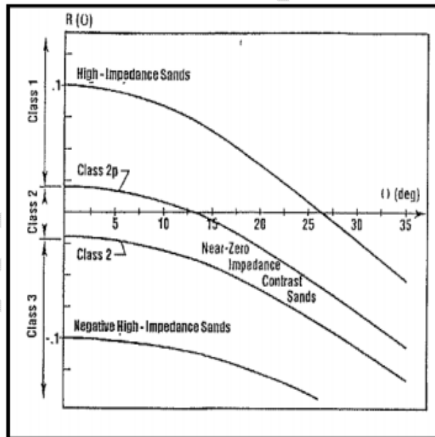
Fig. 4. Anomaly amplitude classification showing the two types of Class 2 AVO [30, 32]
