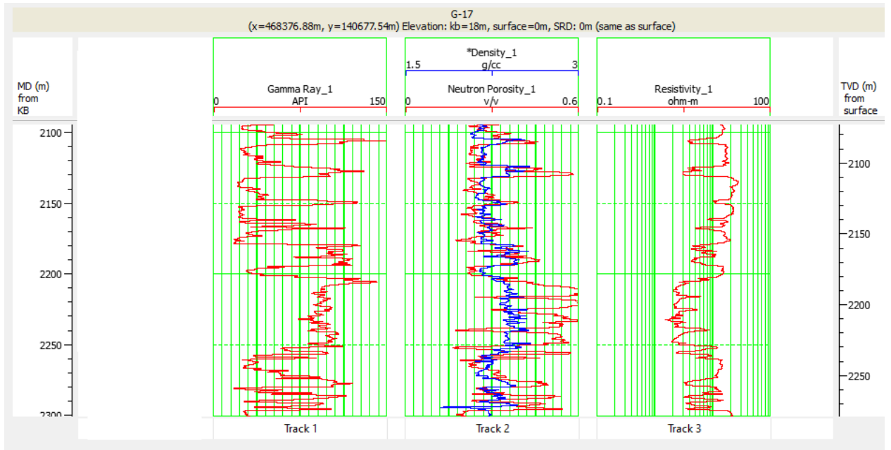
Fig. 8. Typical log section display of raw log suite for G-17.
