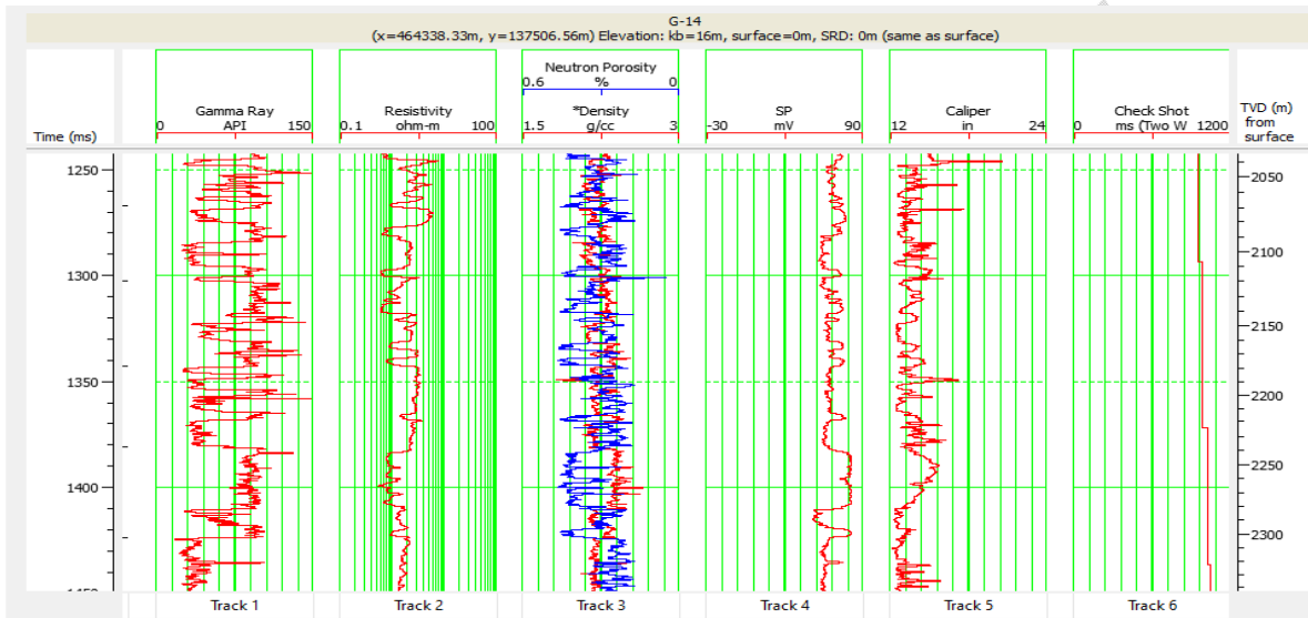
Fig. 5. Typical log section display of raw log suite for G-14.
