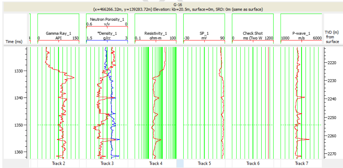
Fig. 7. Typical log section display of raw log suite for G-16.
