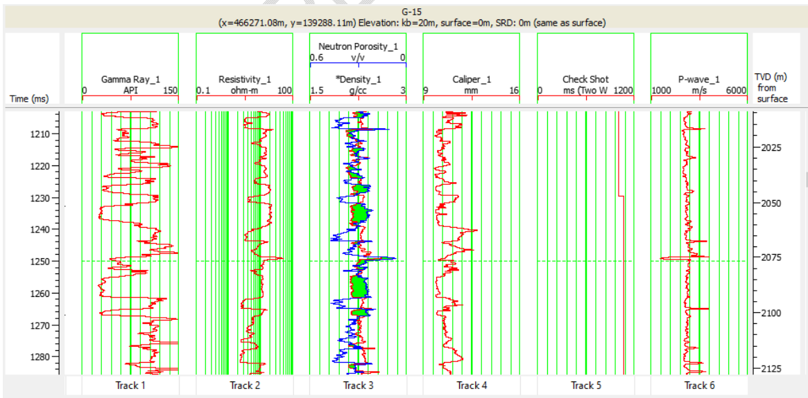
Fig. 6. Typical log section display of raw log suite for G-15.
