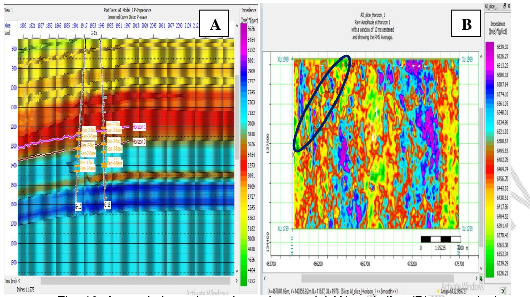
Fig. 19. Acoustic Impedance Inversion model (A) and slice (B) respectively
