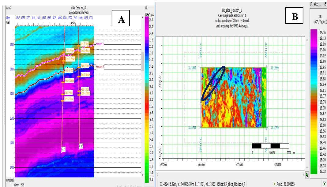
Fig. 21. Lamba rho Inversion model (A) and slice (B)
