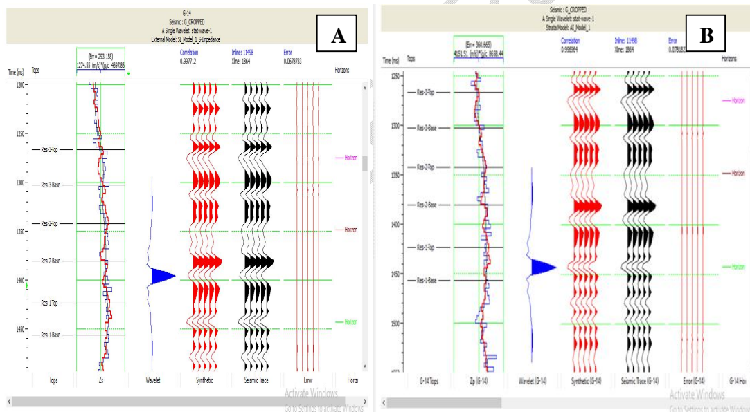
Fig. 18. Post Stack Inversion Analysis at well location showing a good correlation between initial model (A); inverted results (B).
