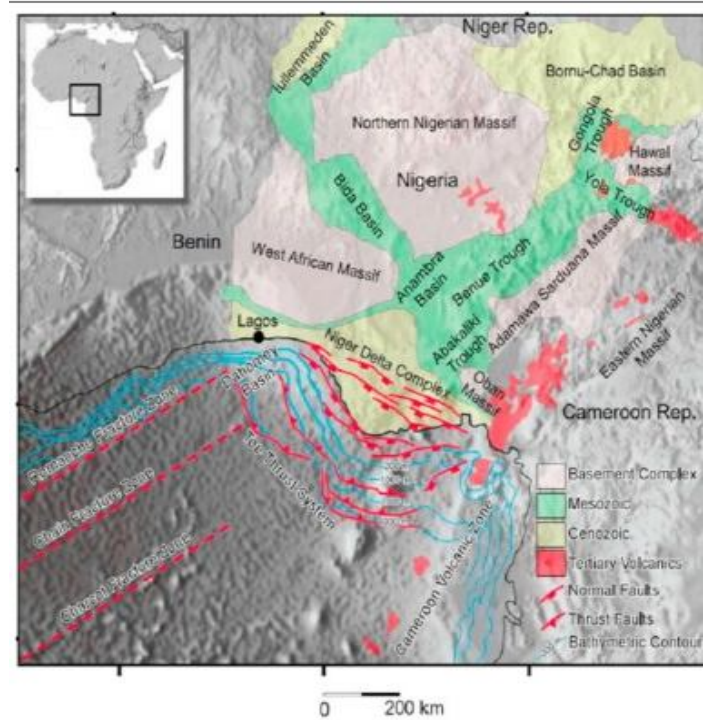
Fig. 2. Niger Delta map showing the main sedimentary basins and tectonic features [22].
