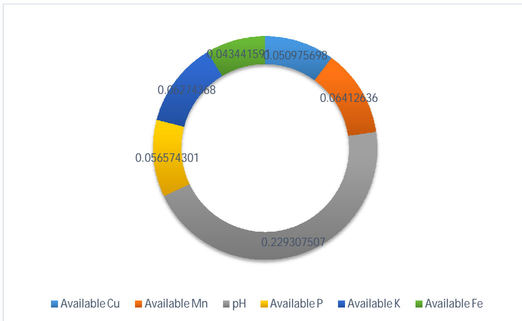
Fig 4: Contributions of significant soil parameters to SQI (Warangal)
