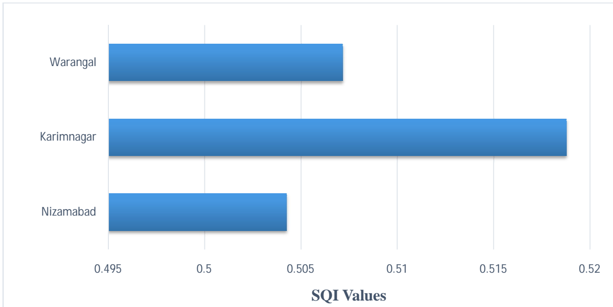
Fig 3: Soil quality index (SQI) in selected districts of Kaleshwaram project area of Telangana state
