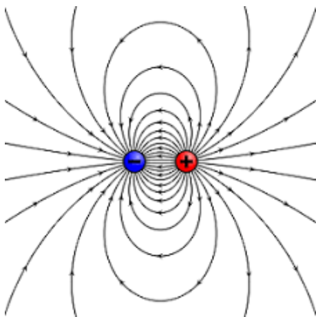
Fig. 3 Illustration of Electric dipole
