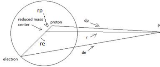
Fig.1 Illustration of Hydrogen Atom
