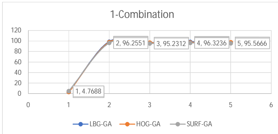
Figure 13: Performance Evaluation of LBP-GA, HOG-GA and SURF-GA for MNIST Digit Document
