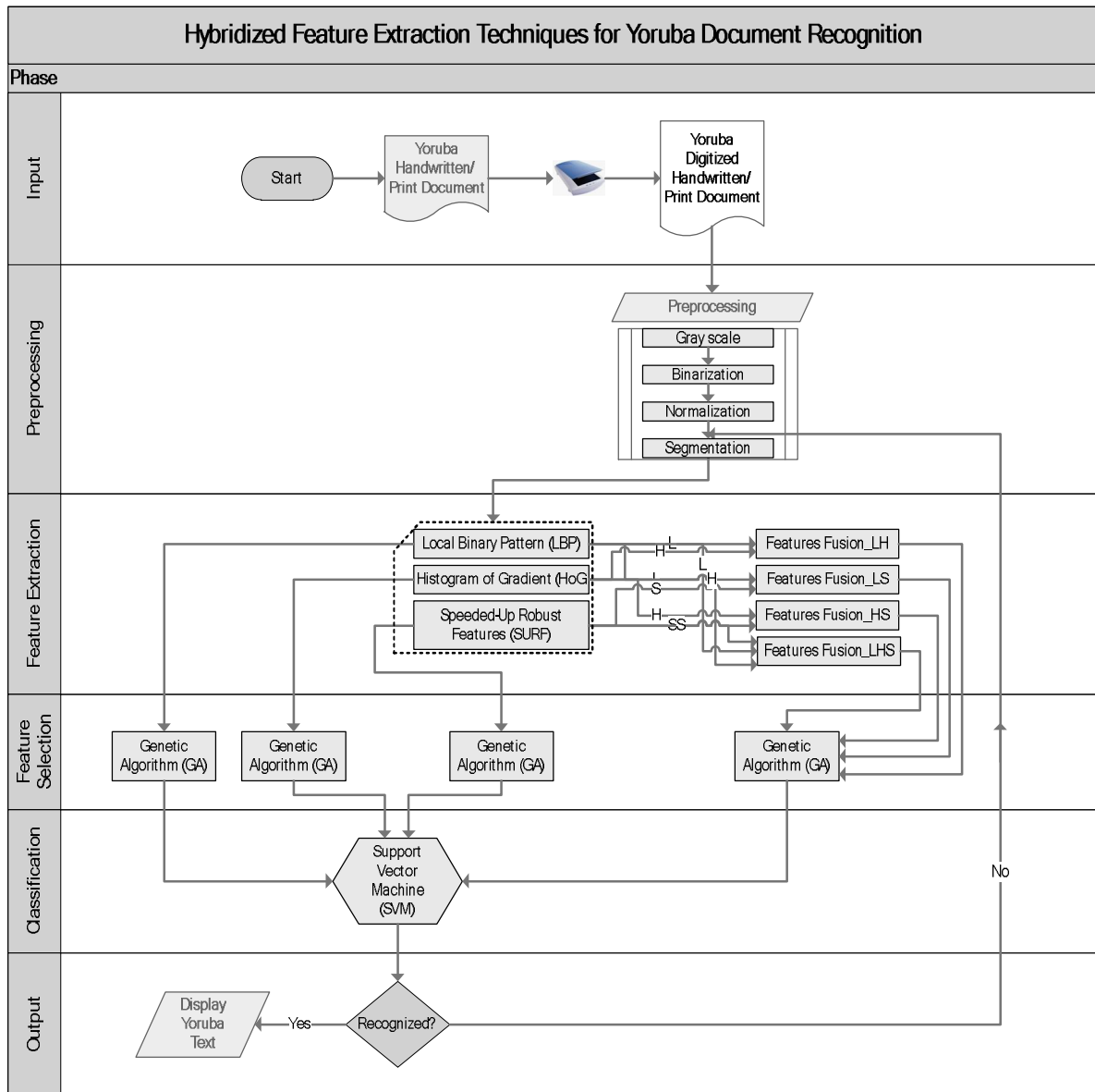
Figure 3: Developed model for the hybridized features extraction techniques
