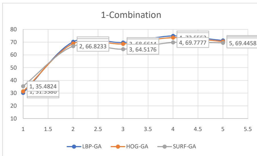
Figure 7: Performance Evaluation of LBP-GA, HOG-GA and SURF-GA for Handwritten Yorùbá Document
