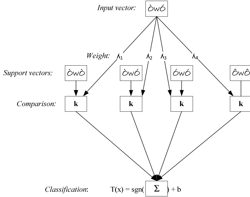
Figure 3: SVM model for Yorùbá document recognition (Source: adapted from [26]).
