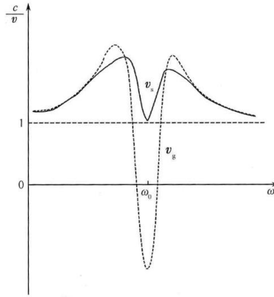
Fig.3 Phase velocity and group velocity in Brillouin theory
