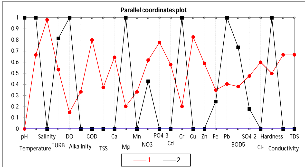
Figure 5: Parallel Coordinate plot
