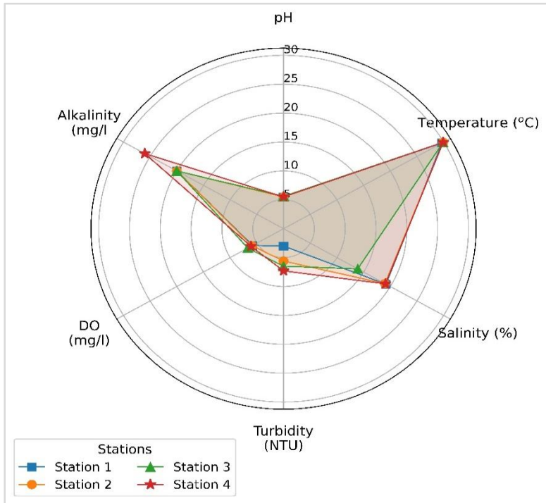
Figure 2: Radar plot showing the physiochemical parameters in the four station
