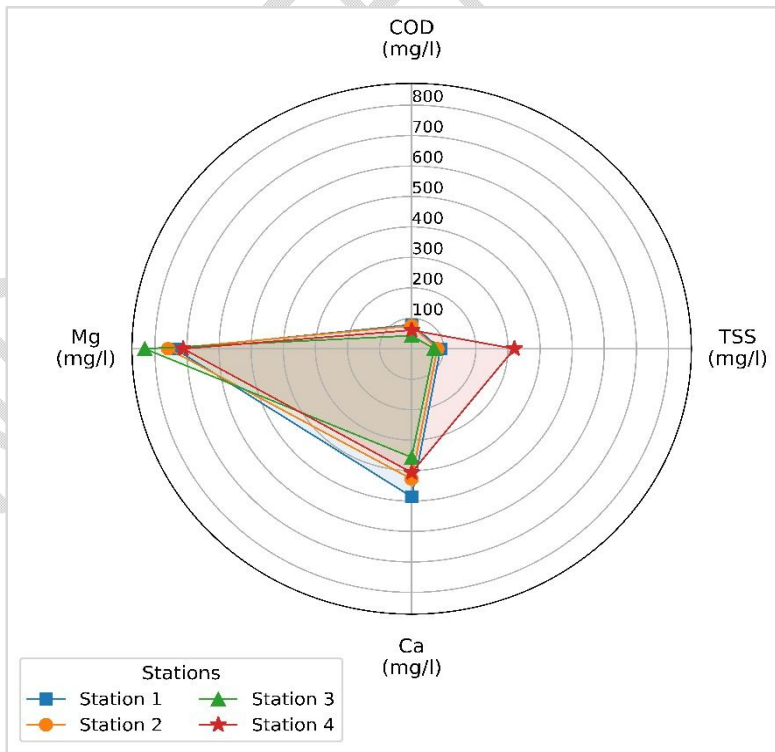
Figure 3: Radar plot showing the physiochemical parameters in the four station
