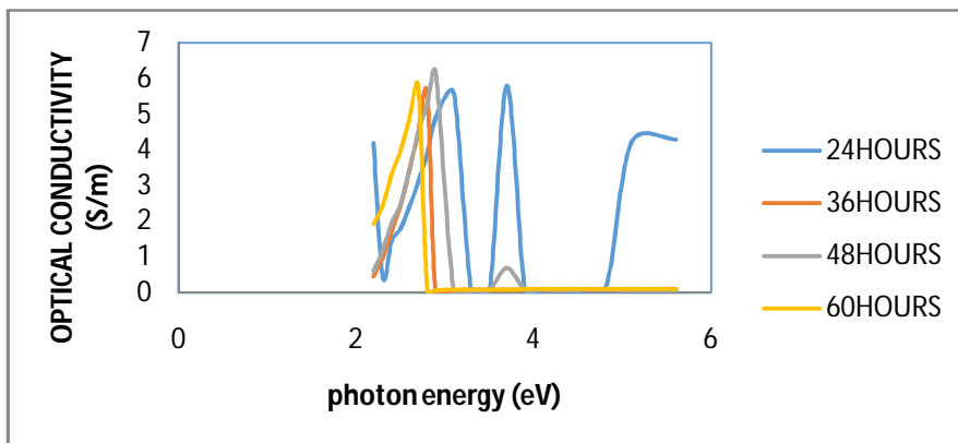
Figure 3.5 plots of optical conductivity against photon energy
