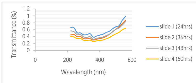
Figure 3.3 plots of transmittance against wavelength for time variation.
