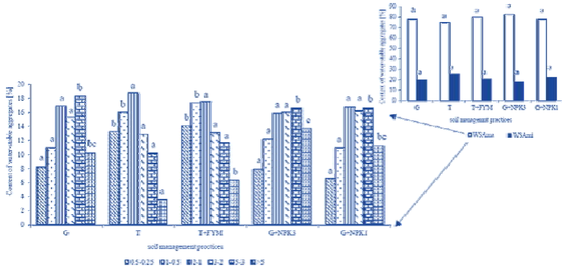
Fig. 1: Water-stable aggregates under diverse soil-management practises: G – control; T – tillage; T+FYM – tillage+ farmyard manure; WSAm and WSAmi are water-stable macro- and micro-aggregates, respectively.
