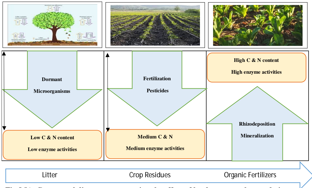
Fig 8(b): Conceptual diagram representing the effect of land use on carbon and nitrogen content in soil
