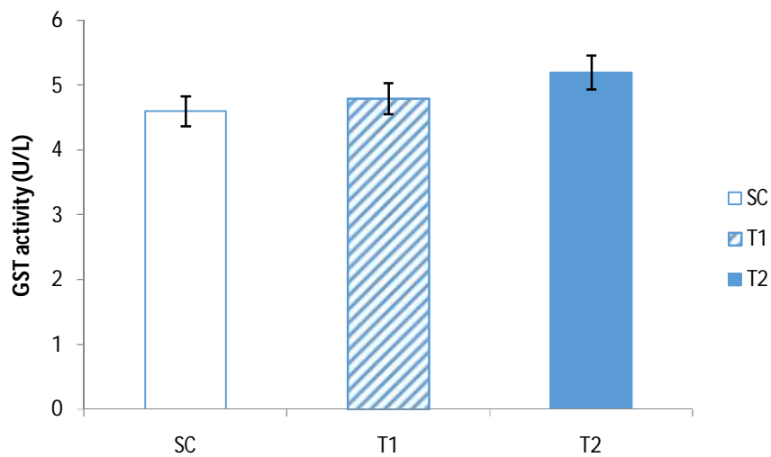
Figure 5: GST activity in fish exposed to ternary PAH mixtures.
