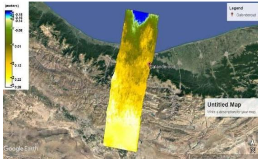
Figure 14: vertical displacement of the first period
