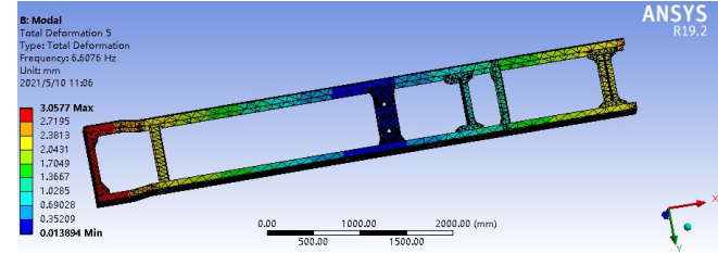
Frame structure 5 natural frequencies
