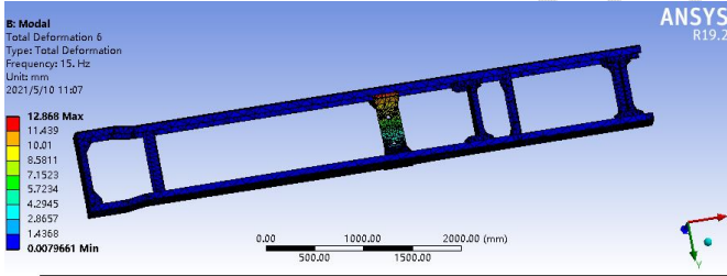
Frame structure 6 natural frequencies
