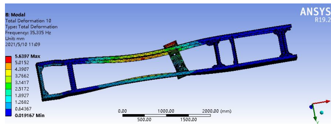
Fig6 First 10 order modal pattern of the frame
