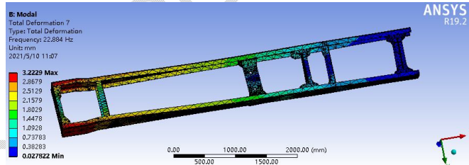
Frame structure 7 natural frequencies
