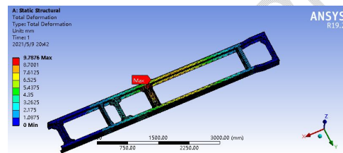
Frame deformation diagram under full load pure bending condition
