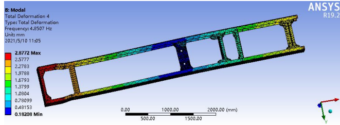
Frame structure 4 natural frequencies
