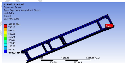
Frame stress diagram under full load pure bending condition
