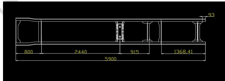
Fig2 dimensional sketch
