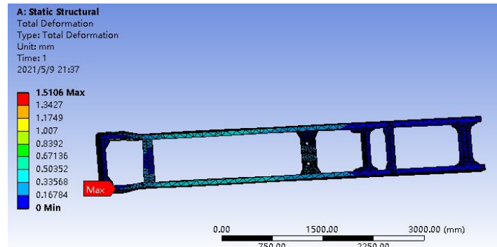
Frame deformation diagram under full load pure bending condition
