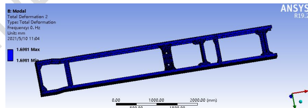
Second order natural frequency of frame structure
