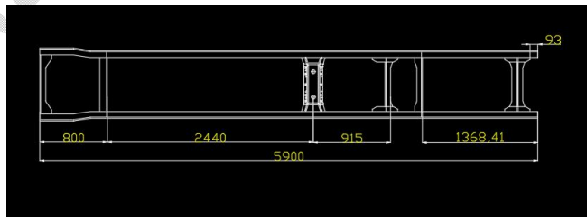
Fig2 dimensional sketch
