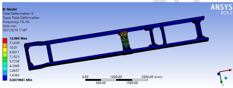
Frame structure 6 natural frequencies
