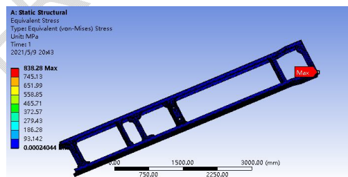
Frame stress diagram under full load pure bending condition
