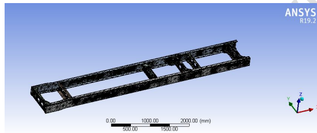
Fig3 mesh model
