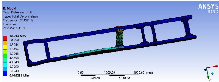
Frame structure 9 natural frequencies
