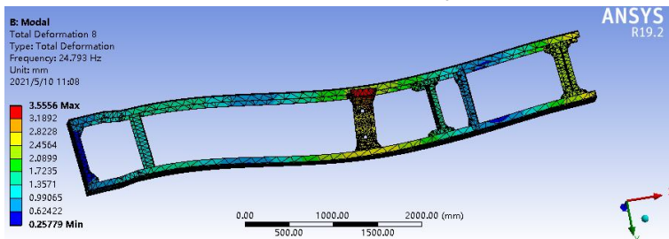
Frame structure 8 natural frequencies
