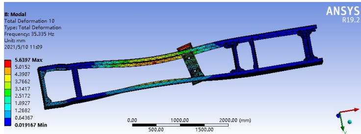
Frame structure 10 natural frequencies
