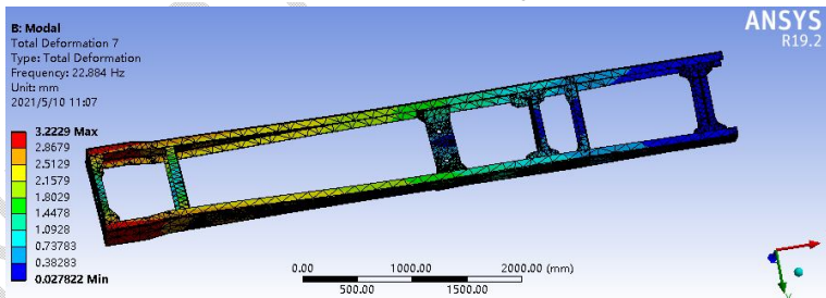
Frame structure 7 natural frequencies
