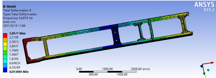
Frame structure 5 natural frequencies
