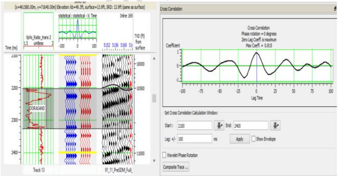
Figure 5: Well -to- Seismic Correlation
