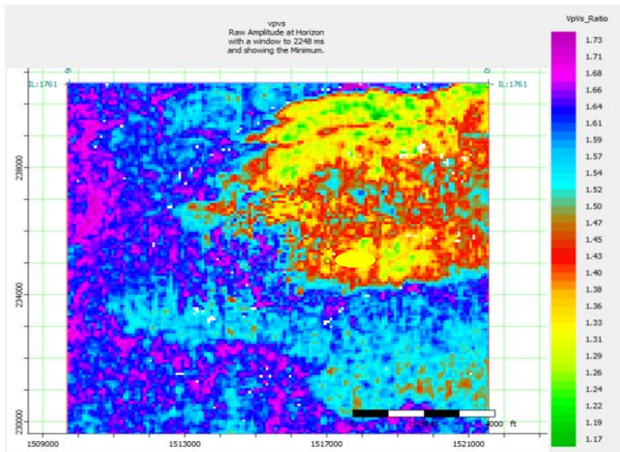
Figure 9: Inverted Vp/Vs Ratio and slice
