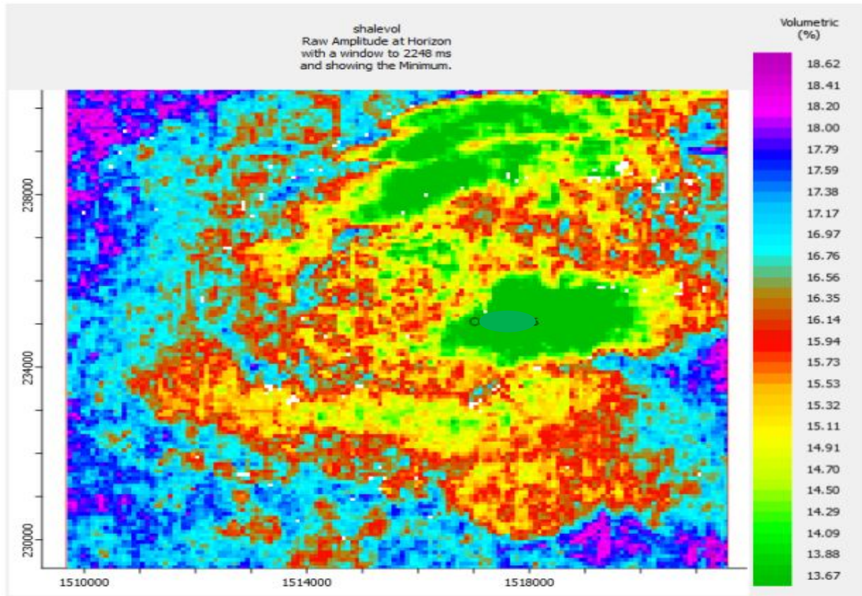
Figure 11: Inverted shale volume and slice
