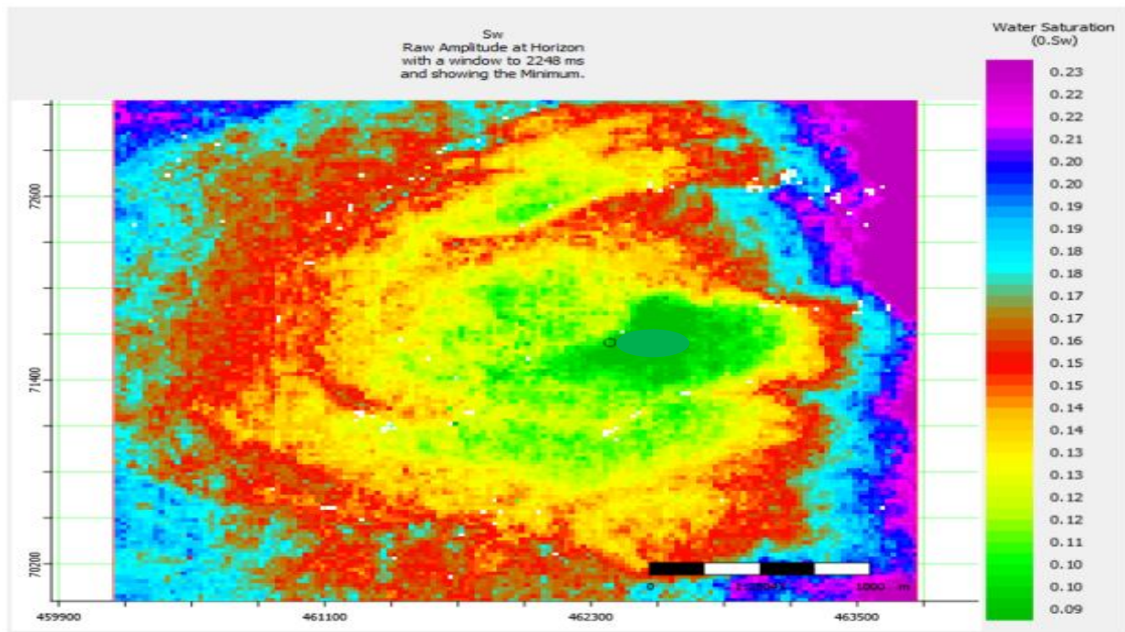
Figure 10: Inverted Water saturation model and slice
