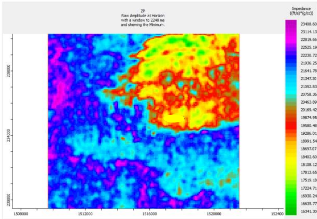
Figure 7: Inverted Acoustic Impedance ( I_p ) and slice
