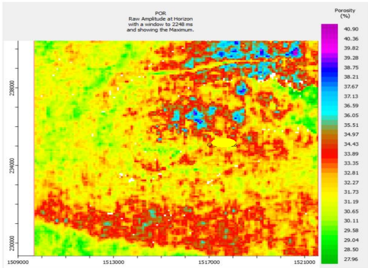
Figure 8: Inverted Porosity and slice
