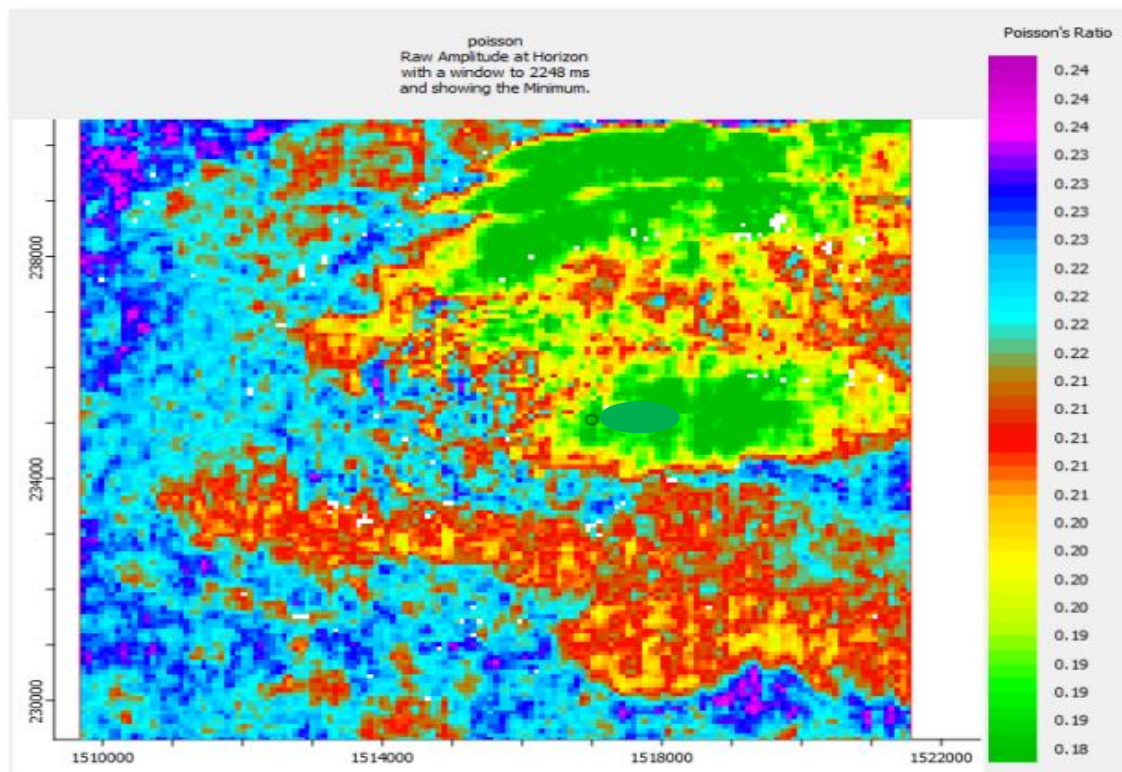
Figure 12: Inverted Poisson ratio and slice
