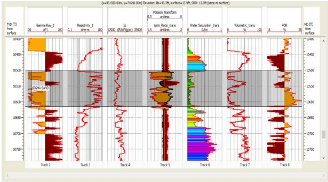
Figure 6: Well log suite of the petrophysical parameters
