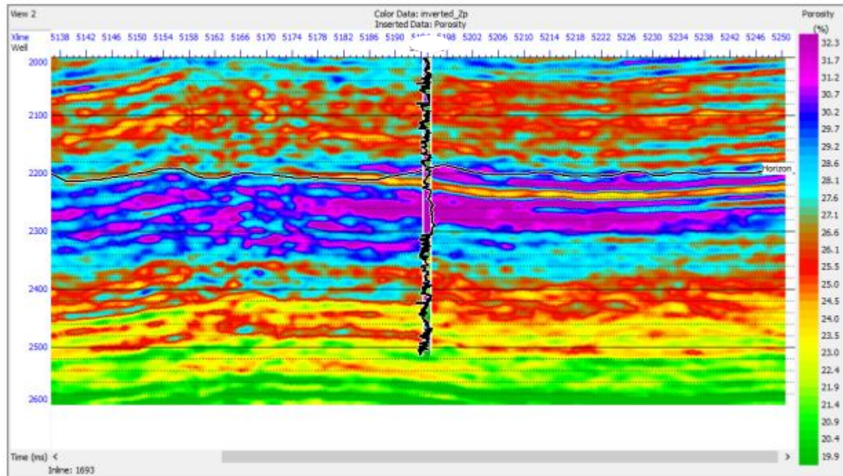
Figure 7: Inverted Acoustic Impedance ( I_p ) and slice
