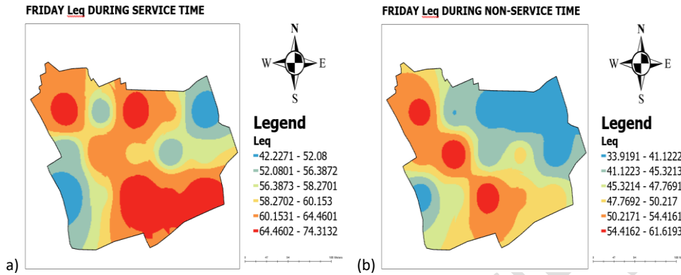
Figure 5: Noise Interpolation Map for Friday L_{eq} during (a) activity time and (b) Non-activity time.
