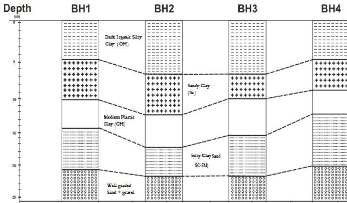
Figure 2: Lithostratigraphy of the Subsurface
