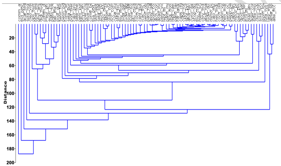
Figure 3: Dendrogram of species on Lapite dumpsite, Ibadan, Oyo State, Nigeria
