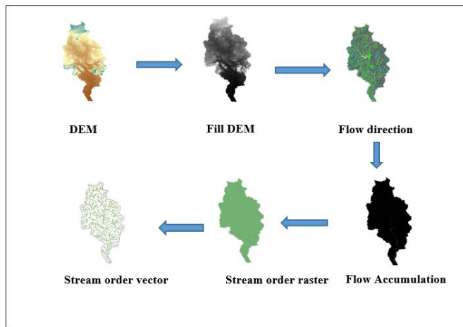
Fig 1. Steps for extraction of drainage network
