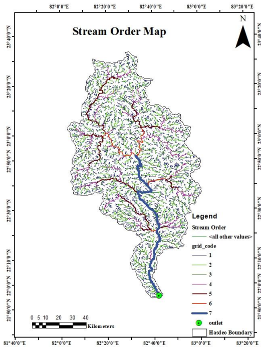
Fig. 3: Drainage network with stream ordering of Hasdeo subbasin
