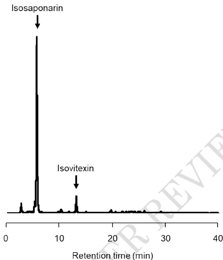
Fig. 6 Chromatogram of HCl-hydrolyzed isosaponarin
