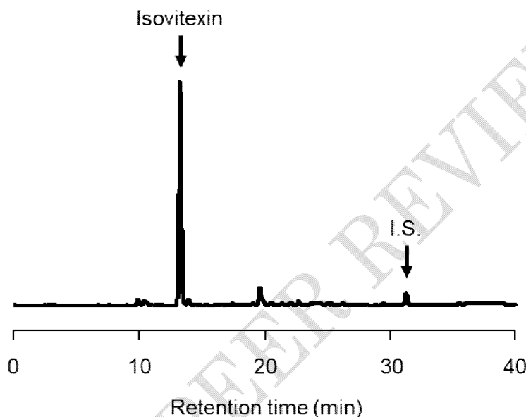
Fig. 5 Representative chromatogram of feces of mice
