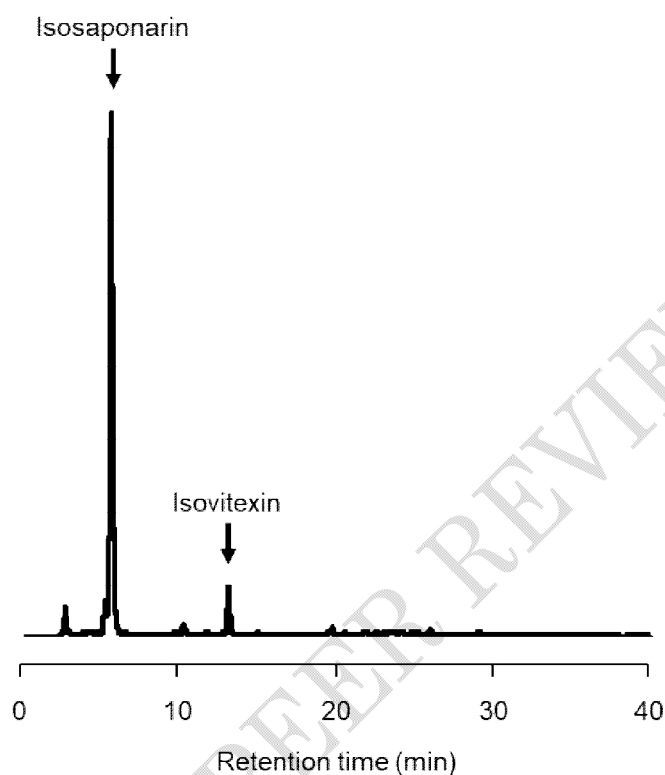
Fig.7 Chromatogram of HCl-hydrolyzed isosaponarin
