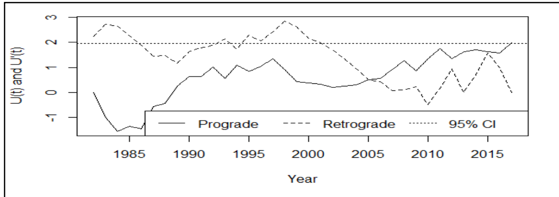
Figure 7: Sequential Mann-Kendall plot for 24-hourly AMS rainfall intensity for Benin
