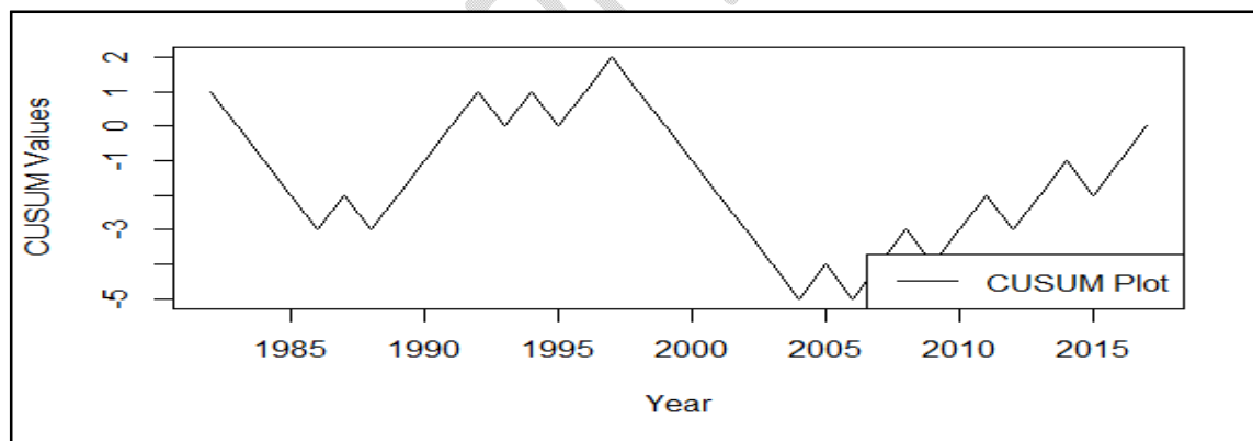
Figure 6: Distribution-free CUSUM plot for 24-hourly AMS rainfall intensity for Benin.
