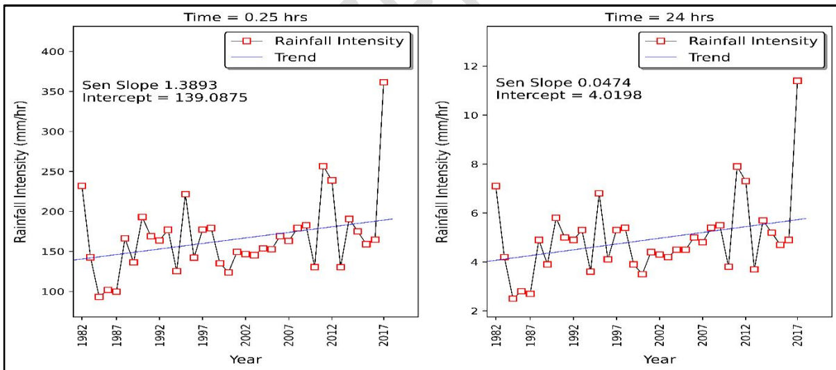
Figure 5: 24-hourly AMS rainfall intensities trend pattern for MCIMD model downscaled durations for Benin City (1982-2017).
