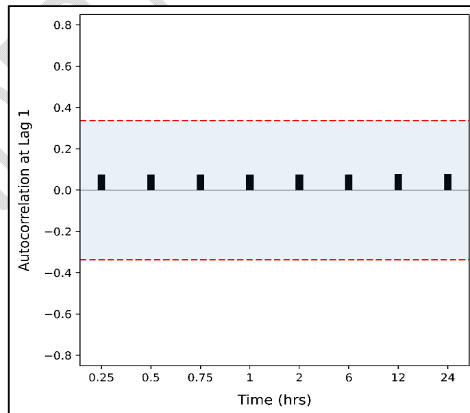
Figure 2: Correlogram of ACF at lag-1 for various 24-hourly AMS downscaled durations using MCIMD model for Benin City.
