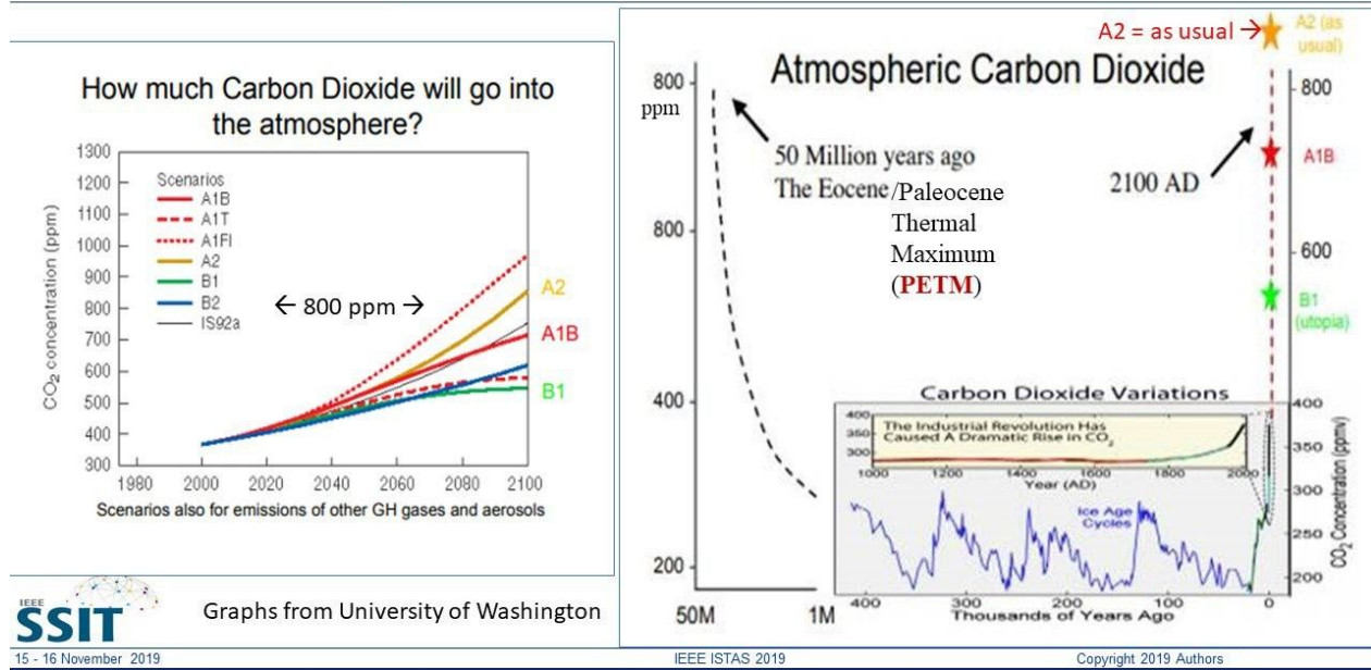
Figure 9 Climate scenario model projections versus paleoclimatology 19
