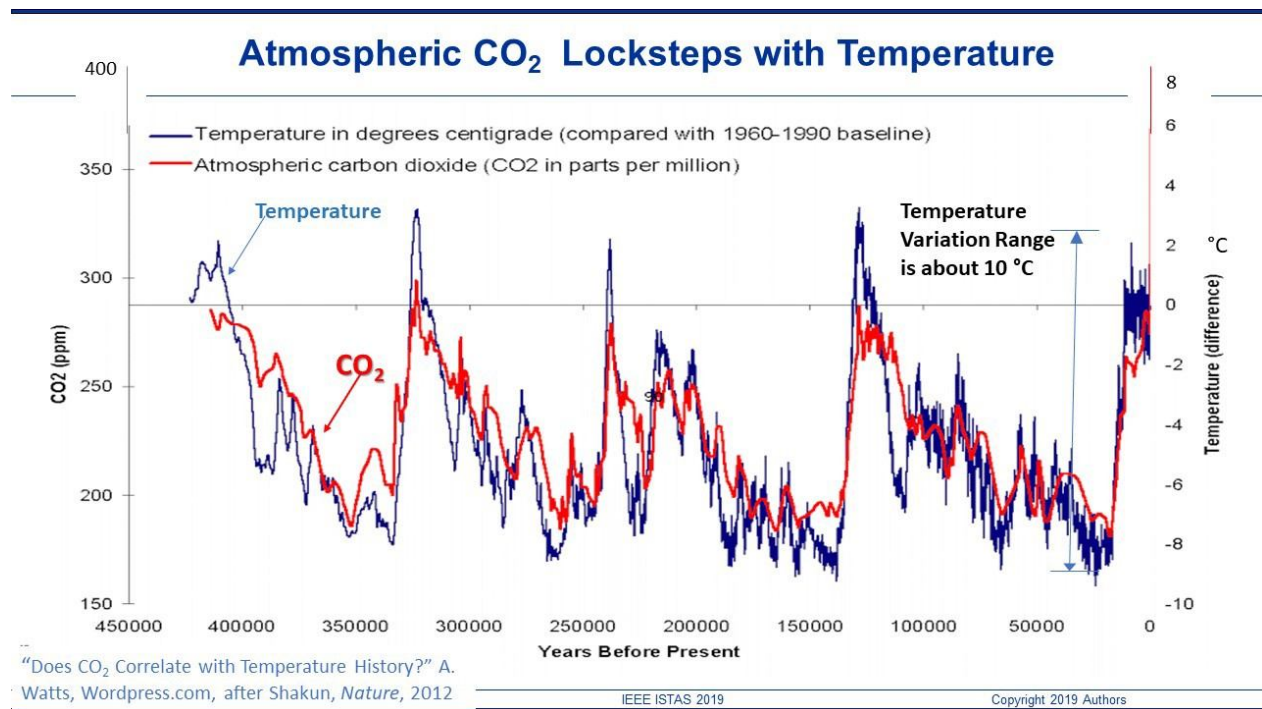
Figure 3 Global average temperature tracks CO 2 levels 5
