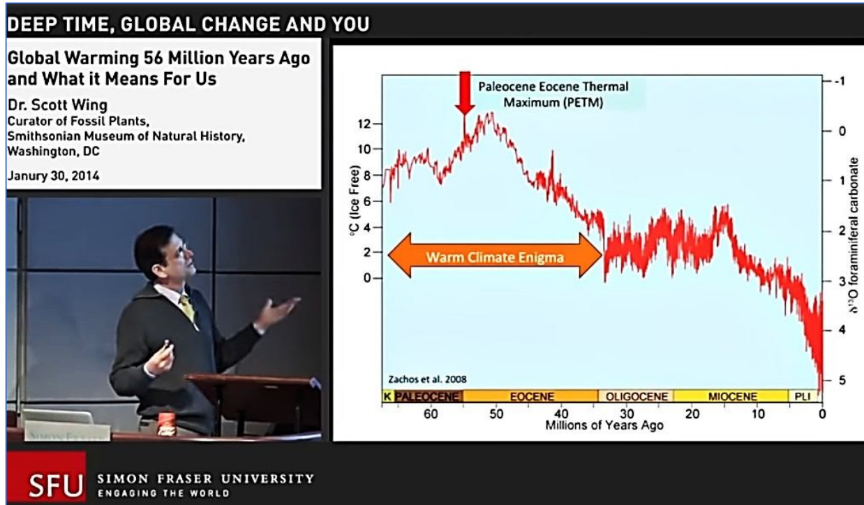
Figure 11 Scott Wing explaining the PETM temperature maximum versus today's global warming climate 29
