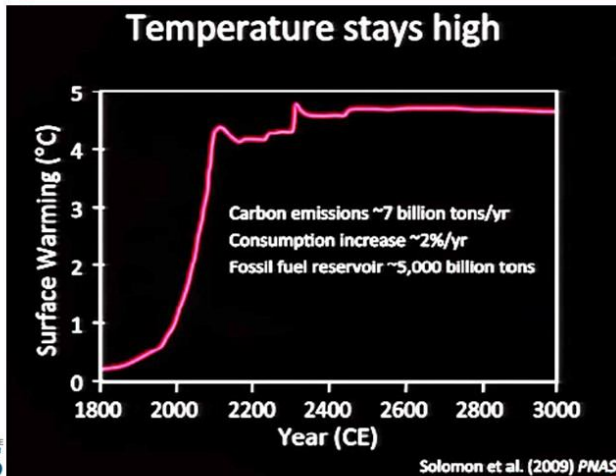
Figure 7 Hansen formula with corroboration by Solomon et al. 11
