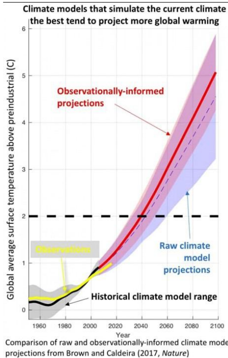
Figure 8 Climate model simulation 14
