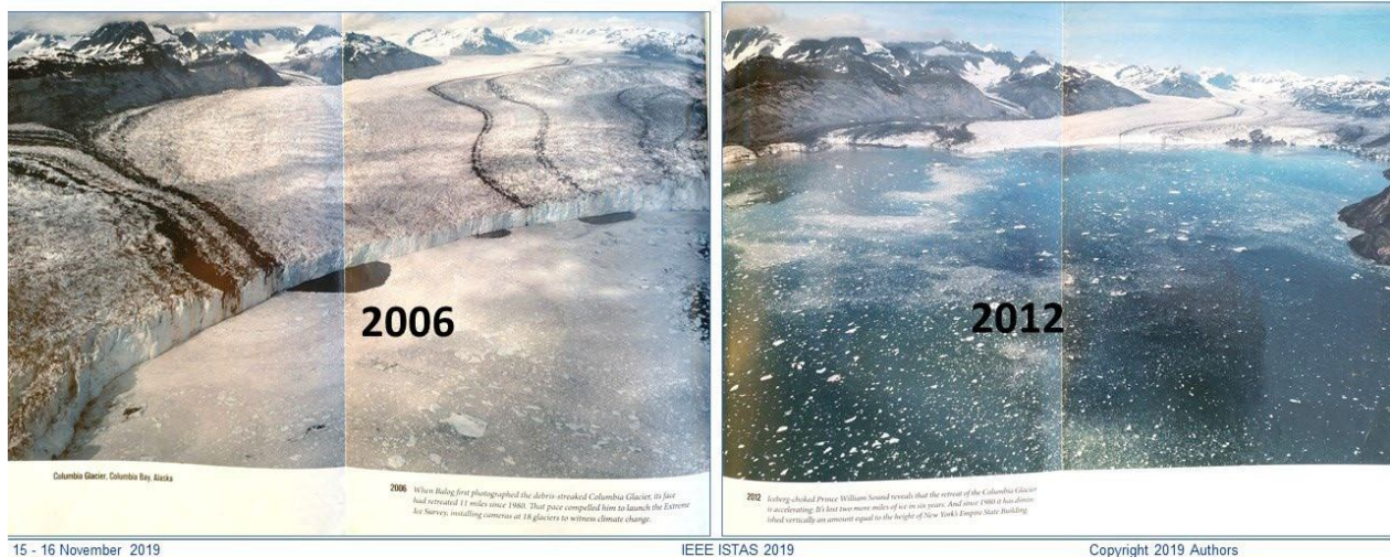
Figure 6 Extreme climatic event 9
