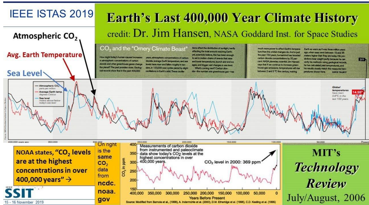
Figure 4 Hansen graph correlating global CO 2 and temperature and sea level 7
