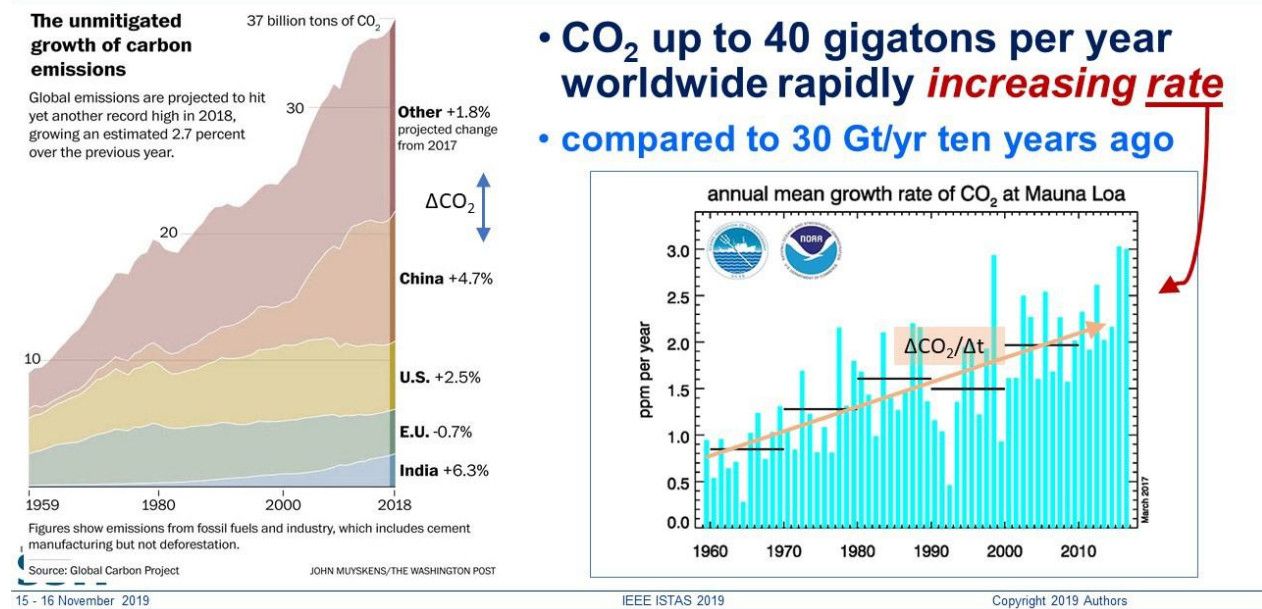
Figure 2 Rate of change for CO 2 emissions per year 4
