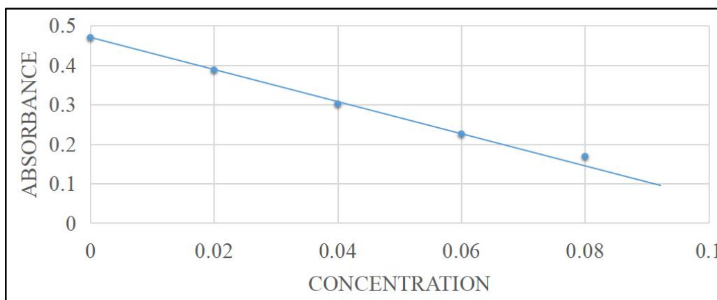
Figure 3: A calibration curve of microgram fluoride versus absorbance relationship
