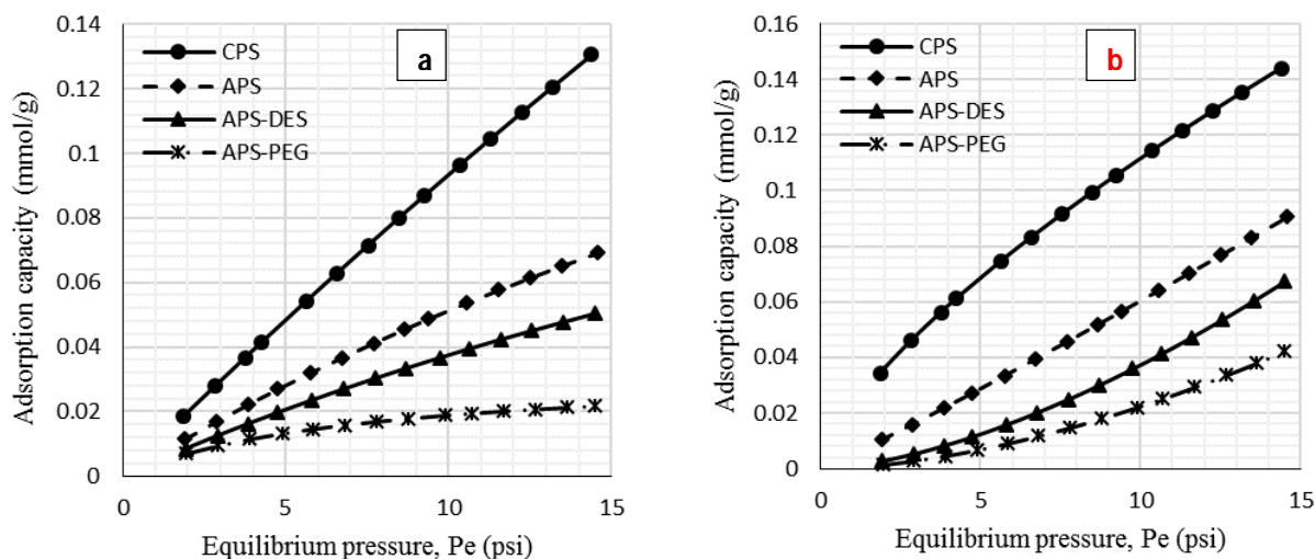
Fig. 5. (a) Langmuir and (b) Freundlich adsorption isotherms
