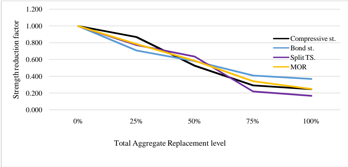
Fig 5. Comparing the reduction factors for the various strength properties of the concrete tested for the concrete mix, P50T50 at different TAR levels.
