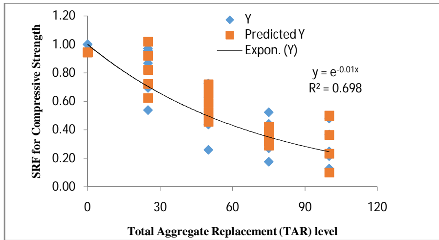
Fig 1. Relationship between SRF for compressive strength and TAR
