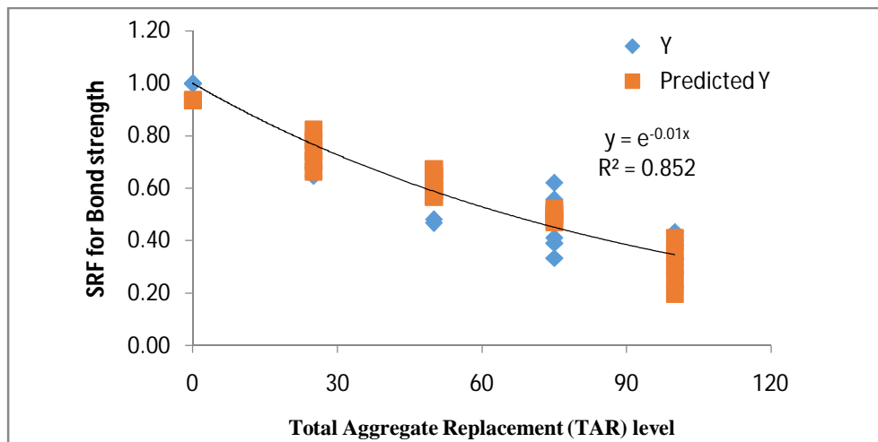
Fig 4. Relationship between SRF for bond strength and TAR
