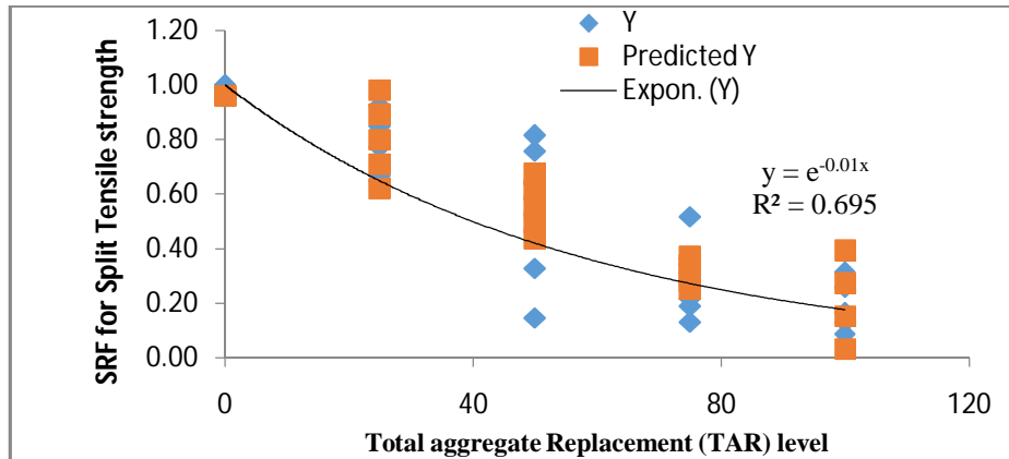
Fig 3. Relationship between SRF for Split Tensile strength and TAR
