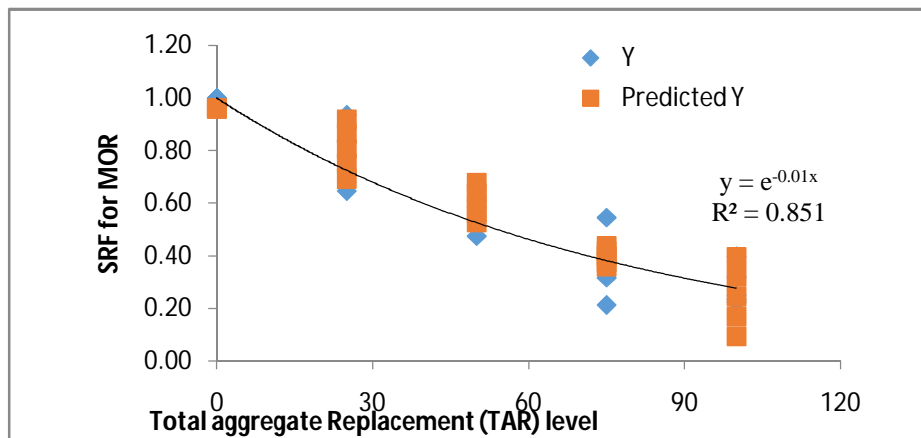
Fig 2. Relationship between SRF for MOR and TAR
