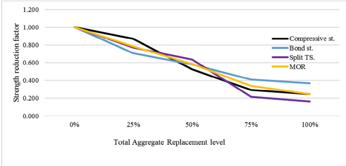
Fig 5. Comparing the reduction factors for the various strength properties of the concrete for the concrete mix, P50T50 at different TAR levels.
