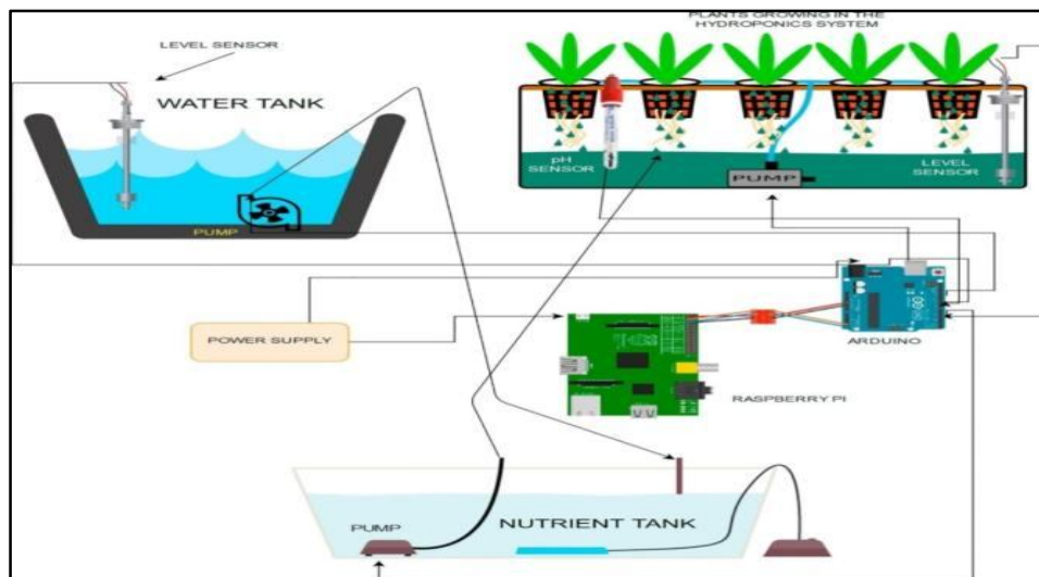
Figure 5: Hydroponics based on IoT (adapted from Mehra et al. , 2018).
