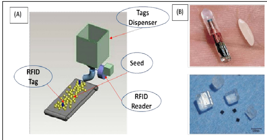
Figure 8: (A) RFID tracking technology for seeds, (B) Examples of RFID tags whose size is comparable to the size of rice (modified from Hornbaker et al. , 2004).
