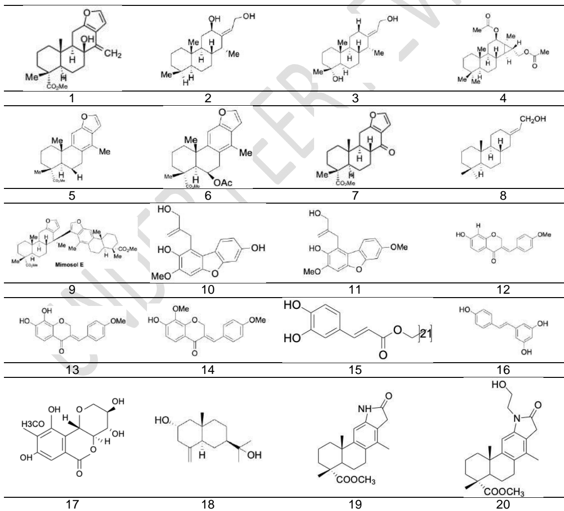
Fig. 1. Molecular structure of above chemical compounds
