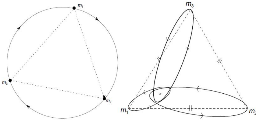
Figure 2: The Lagrange solution: the three bodies form an equilateral triangle at all times. Left: three equal masses. Right: unequal masses
