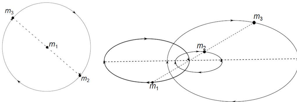
Figure 1: The Euler solution: the three bodies remain collinear at all times, in elliptical orbits around the center of mass. Left: all masses equal. Right: unequal masses
