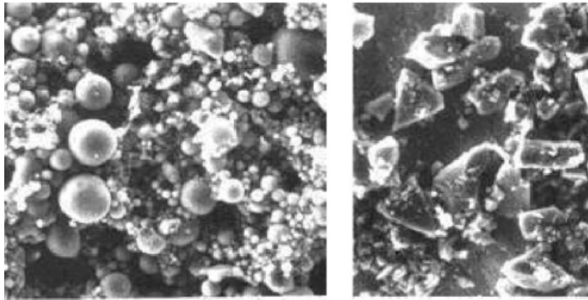
Figure 1 Morphological effect of mineral admixtures
