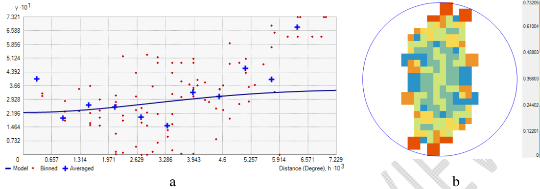
Fig. 3 Experimental semivariogram graph (a) and map (b)
