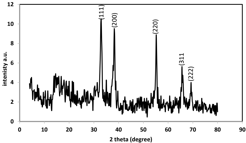
Figure 1. XRD pattern of CdO nanoparticles.
