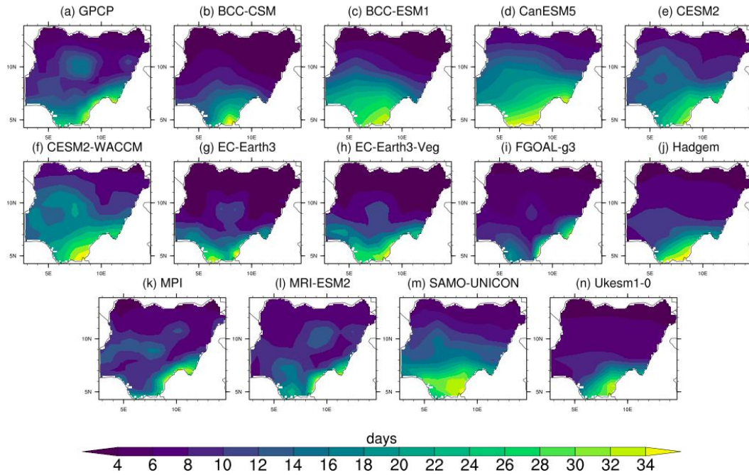
Fig 6. Consecutive wet days (CWD), indicating observation a (GPCP) and b-n (CMIP6 Models)
