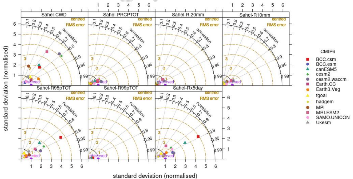
Fig 11. Taylor diagram showing the correlation between GPCP observations and CMIP6 Models.
