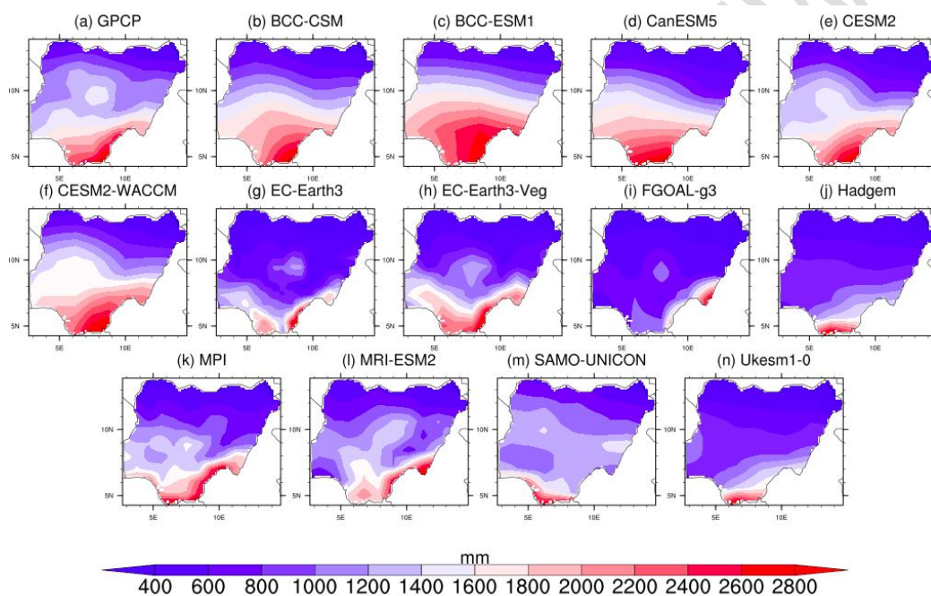
Fig 5. Total wet-day precipitation (PRCPTOT), indicating observation a (GPCP) and b-n (CMIP6 Models)
