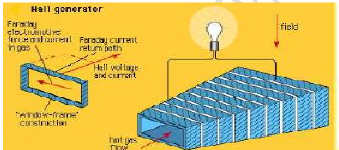
Figure 9: Hall Generator (Bilal et al. , 2014)
