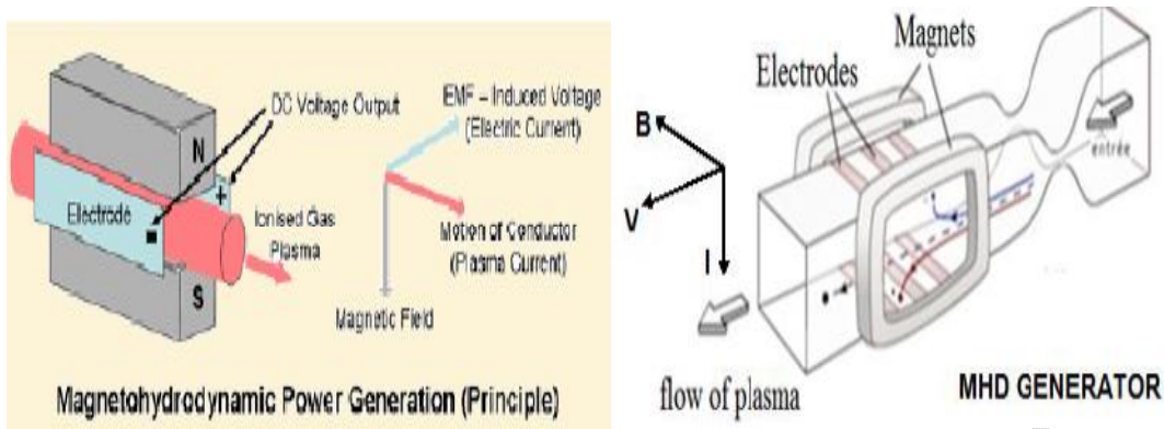
Figure 10: MHD power generation principle (Salvalore and Alessandra, 2014)
