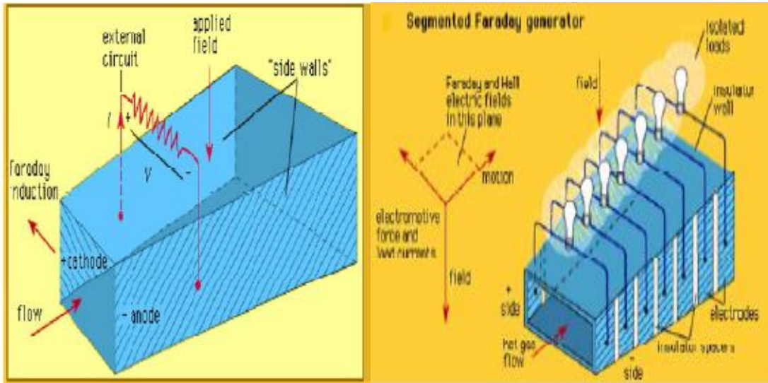
Figure 8: Segmented Faraday Generator (Bilal et al. , 2014)
