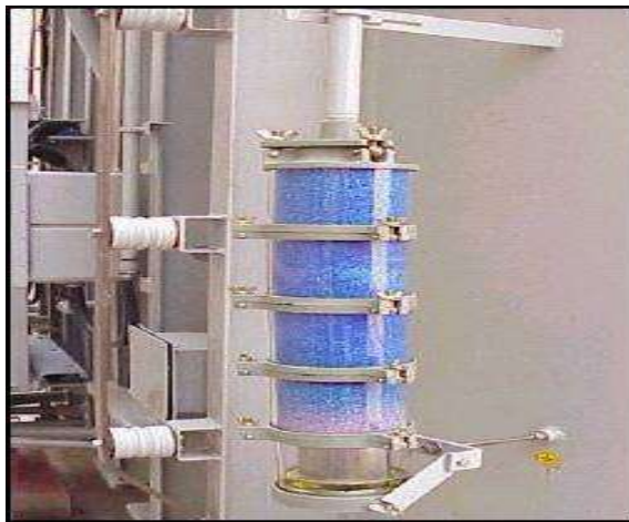
FIG. 3 the transformer respirator [10]
