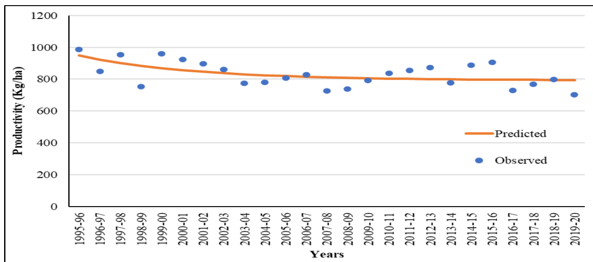
Fig. 3: Observed and predicted values of Productivity of Coffee in Chikkamagaluru district by Gompertz model for the period from 1995-96 to 2019-20.
